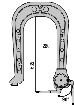
SHARK A7 ARM + ELECTRODE L=635 mm - ● 803189
